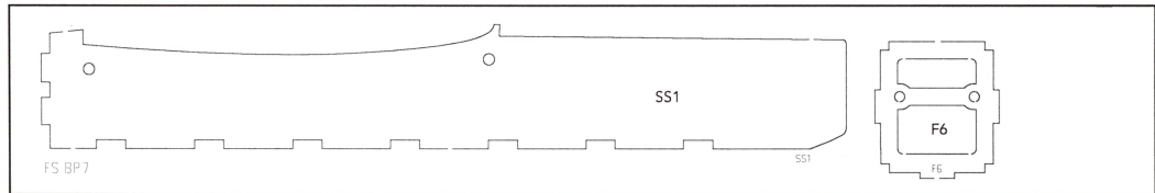
BP7 3/32" Balsa
